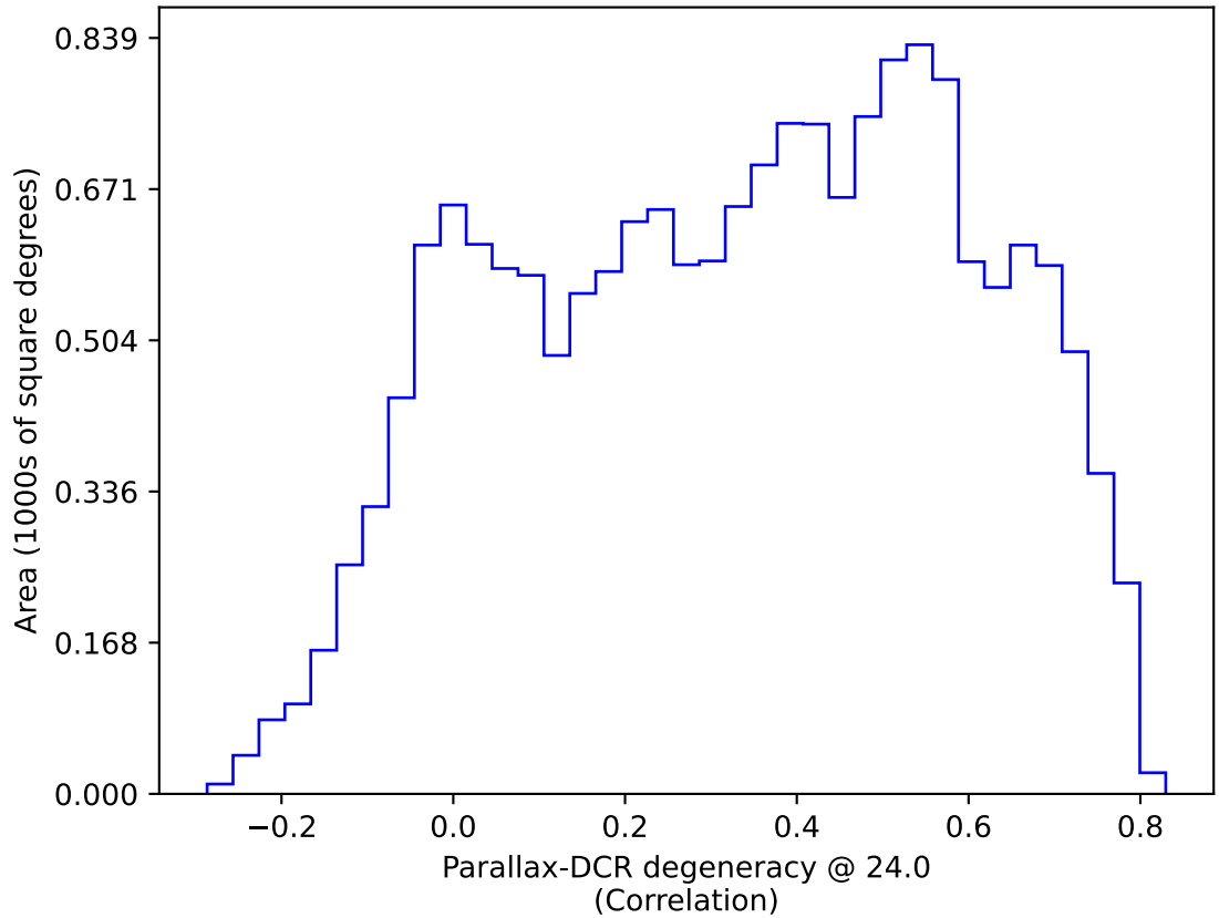
too_elab_heavy_r32_d3_griz_v3.4_10yrs WFD: Parallax-DCR degeneracy @ 24.0
