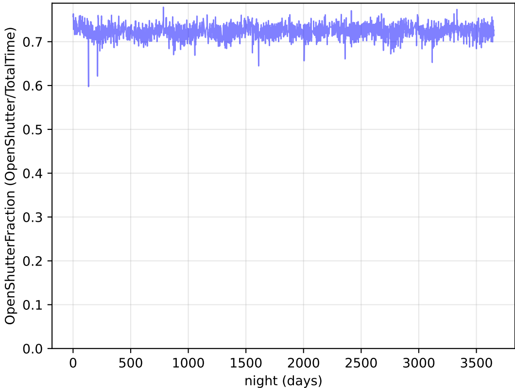
too_elab_heavy_r32_d3_griz_v3.4_10yrs Per night: OpenShutterFraction
