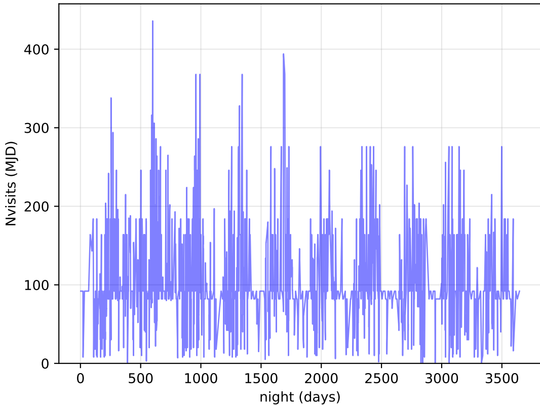
too_elab_heavy_r32_d3_griz_v3.4_10yrs DDF: Nvisits
