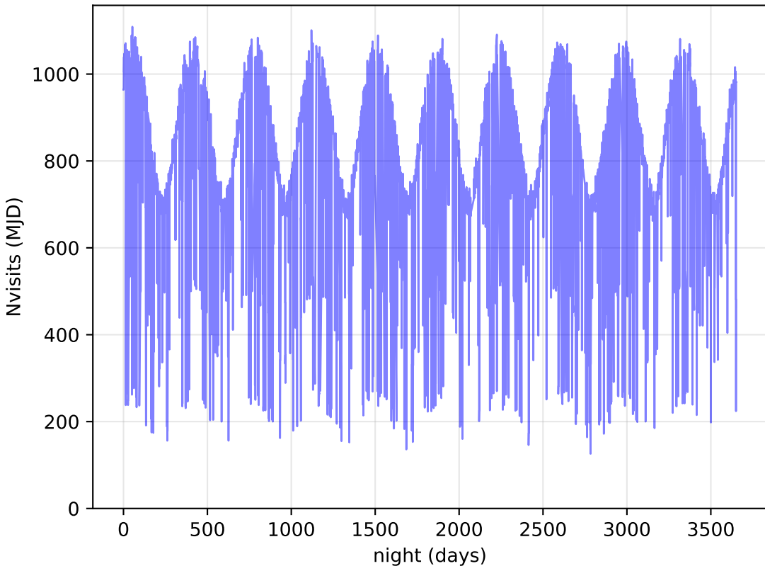
too_elab_heavy_r32_d3_griz_v3.4_10yrs All visits: Nvisits
