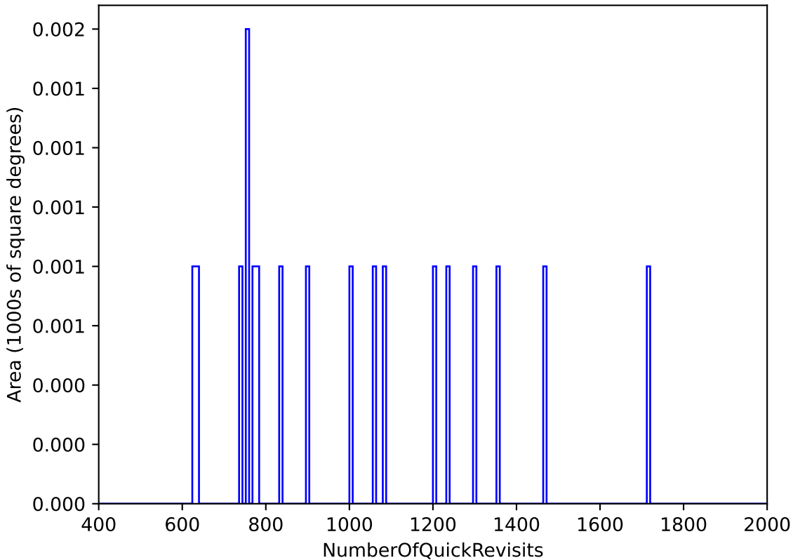
too_elab_heavy_r32_d3_griz_v3.4_10yrs WFD: NumberOfQuickRevisits
