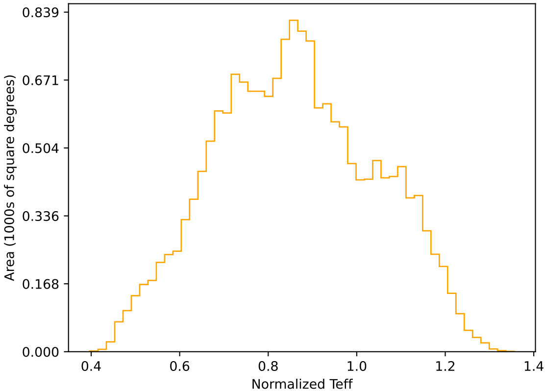
too_elab_heavy_r32_d3_griz_v3.4_10yrs WFD r band: Normalized Teff
