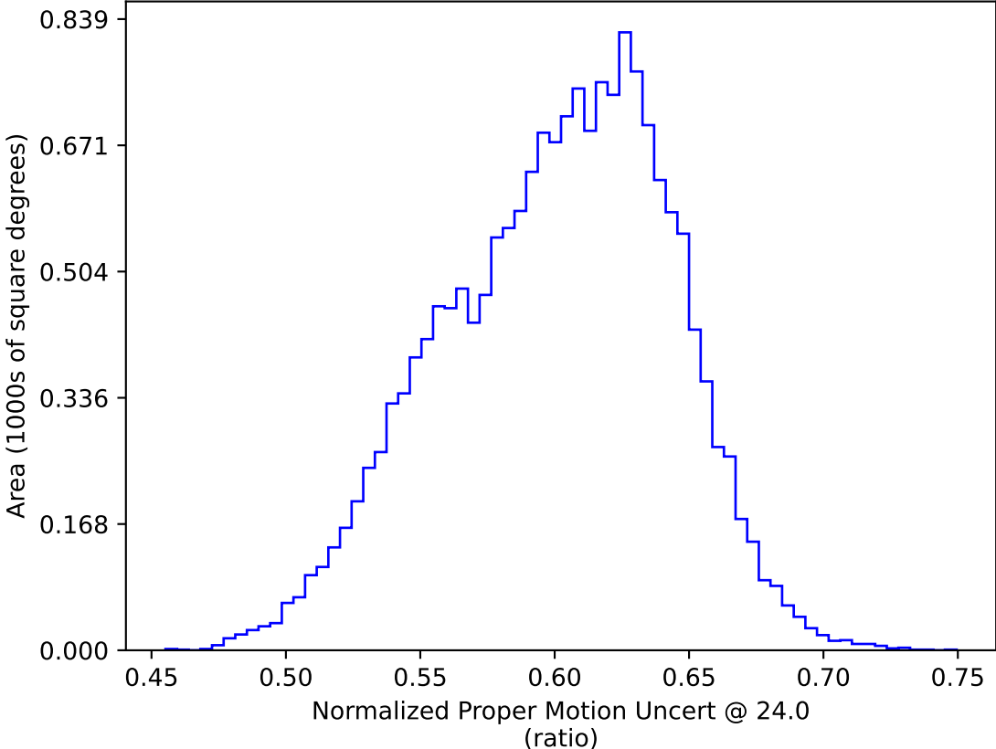
too_elab_heavy_r32_d3_griz_v3.4_10yrs WFD: Normalized Proper Motion Uncert @ 24.0
