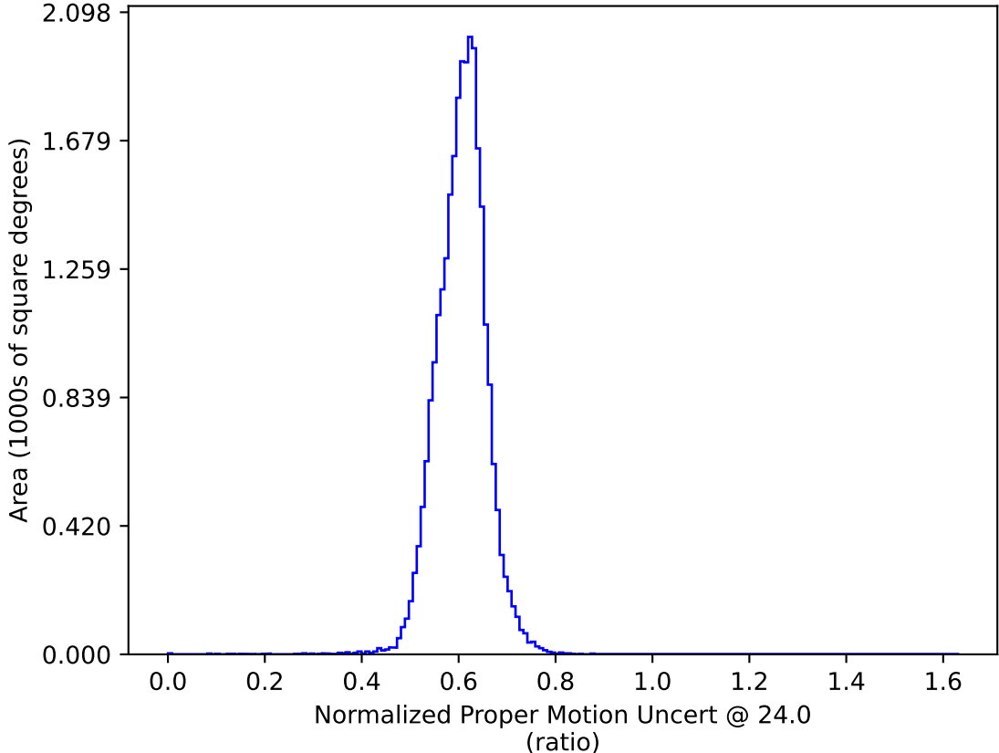
too_elab_heavy_r32_d3_griz_v3.4_10yrs All sky: Normalized Proper Motion Uncert @ 24.0
