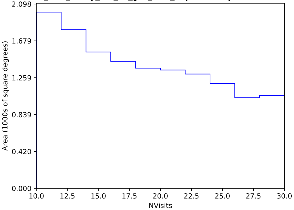
too_elab_heavy_r32_d3_griz_v3.4_10yrs Yr 3-4 y band: NVisits
