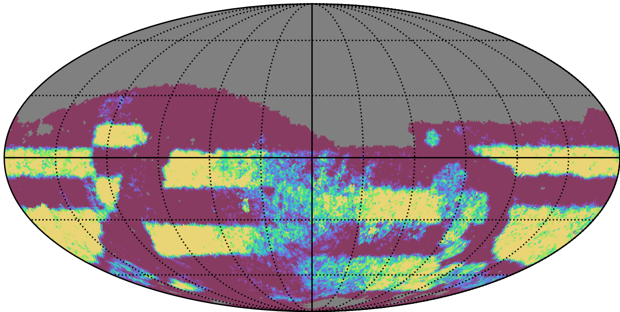
too_elab_heavy_r32_d3_griz_v3.4_10yrs Yr 3-4 r band: NVisits
