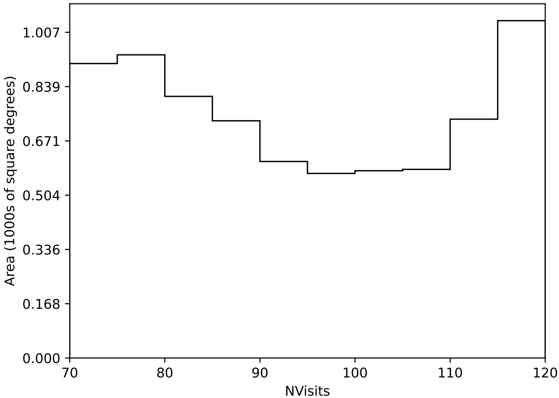
too_elab_heavy_r32_d3_griz_v3.4_10yrs Yr 3-4 all bands: NVisits
