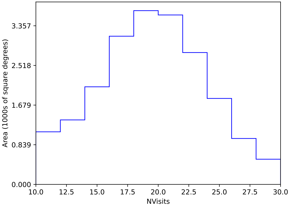
too_elab_heavy_r32_d3_griz_v3.4_10yrs Yr 1 y band: NVisits
