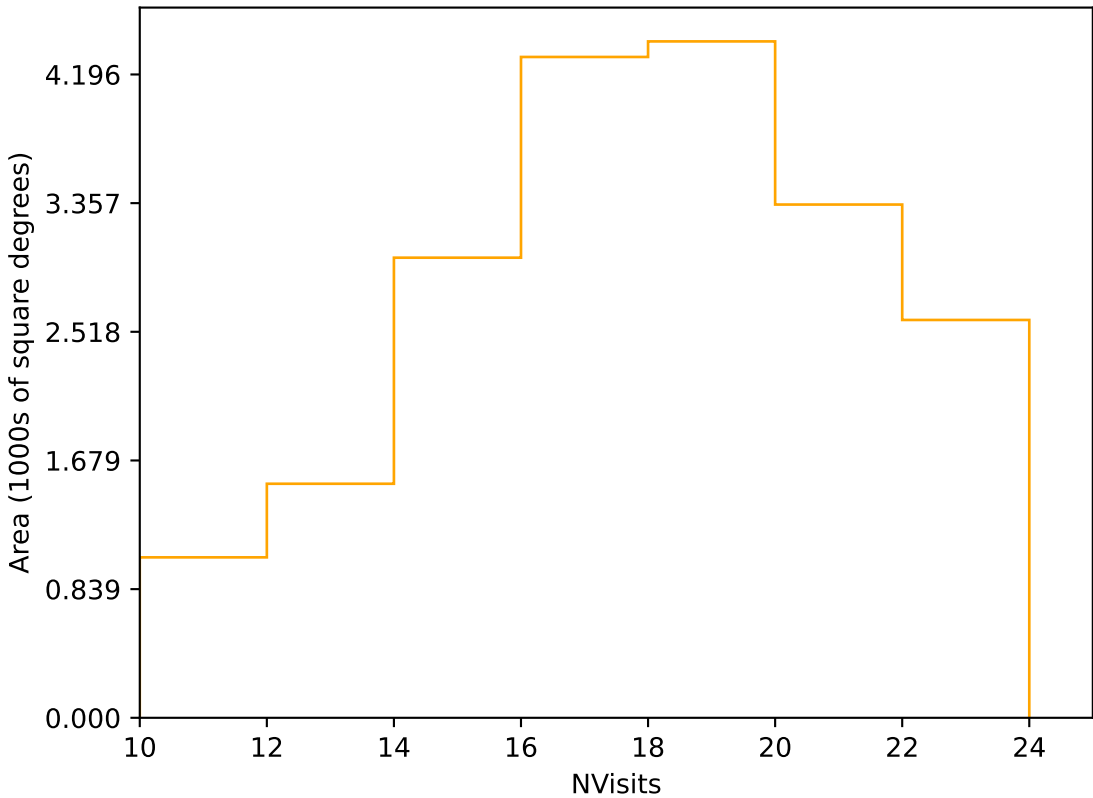
too_elab_heavy_r32_d3_griz_v3.4_10yrs Yr 1 r band: NVisits
