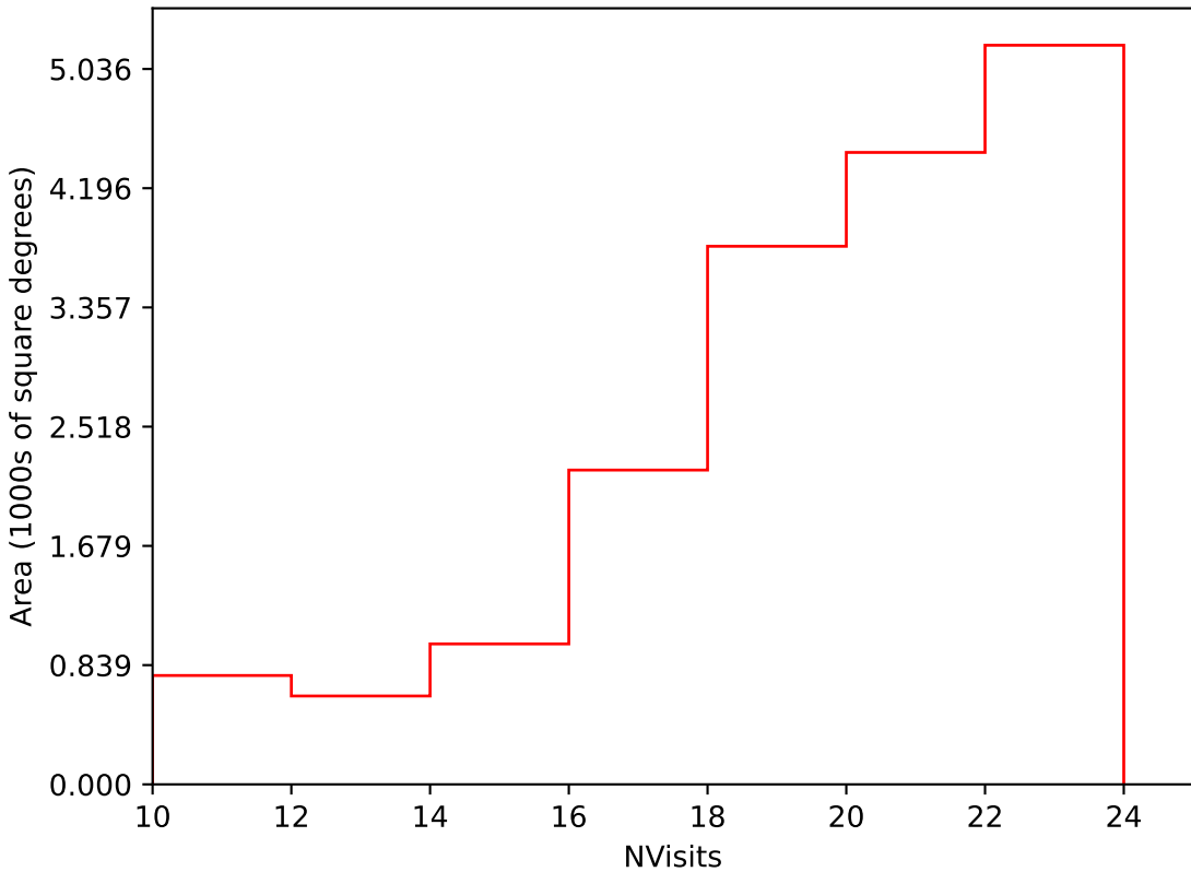
too_elab_heavy_r32_d3_griz_v3.4_10yrs Yr 1 i band: NVisits
