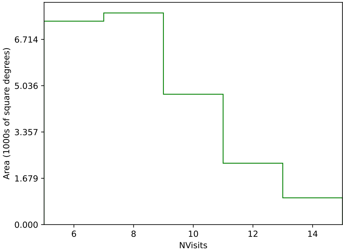
too_elab_heavy_r32_d3_griz_v3.4_10yrs Yr 1 g band: NVisits
