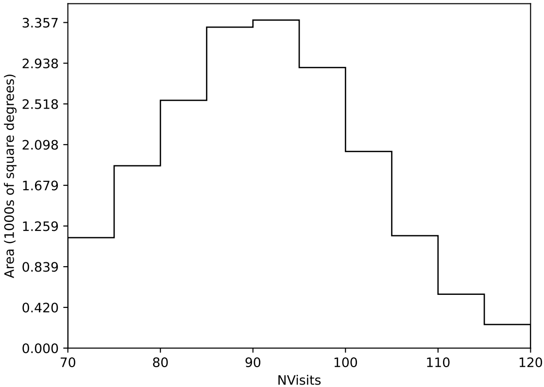
too_elab_heavy_r32_d3_griz_v3.4_10yrs Yr 1 all bands: NVisits
