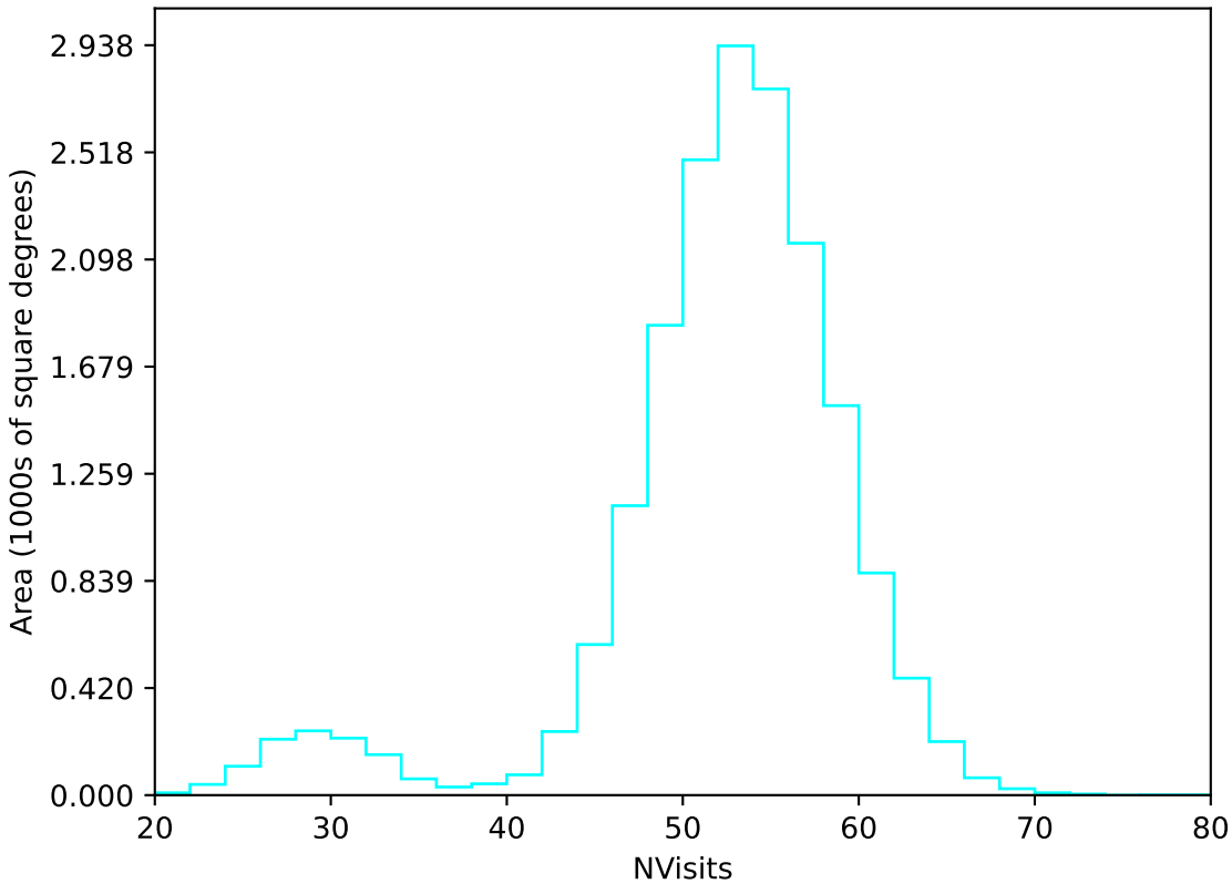
too_elab_heavy_r32_d3_griz_v3.4_10yrs WFD u band: NVisits
