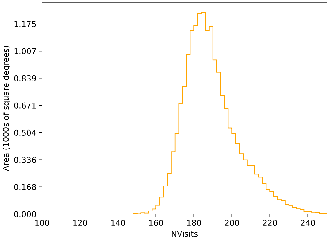
too_elab_heavy_r32_d3_griz_v3.4_10yrs WFD r band: NVisits
