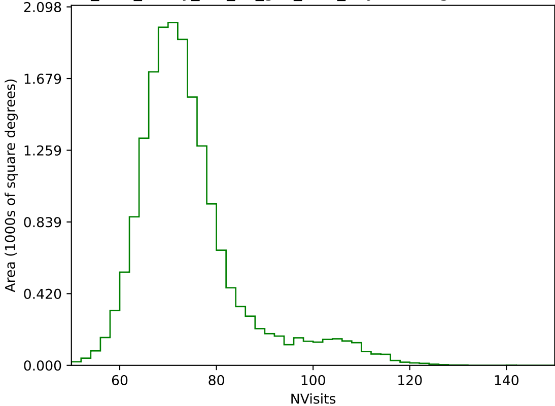
too_elab_heavy_r32_d3_griz_v3.4_10yrs WFD g band: NVisits
