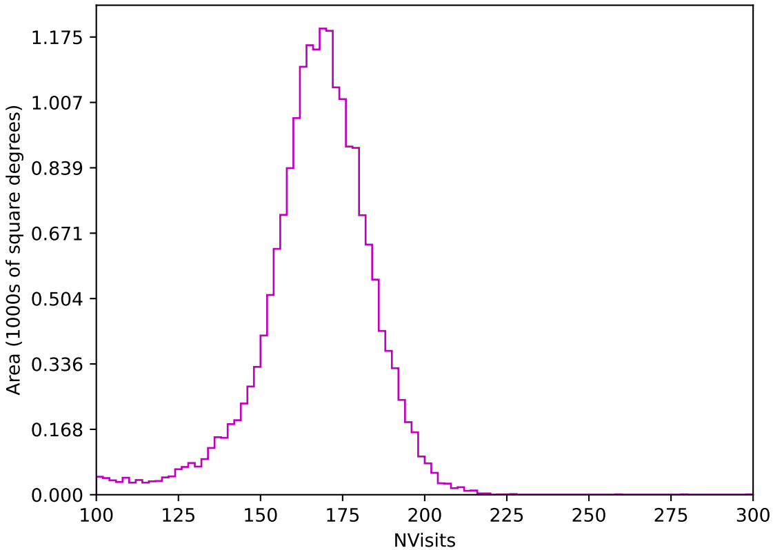
too_elab_heavy_r32_d3_griz_v3.4_10yrs All sky z band: NVisits
