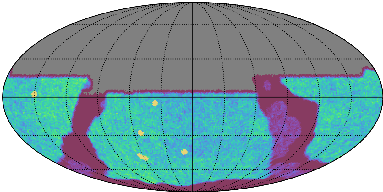
too_elab_heavy_r32_d3_griz_v3.4_10yrs All sky u band: NVisits
