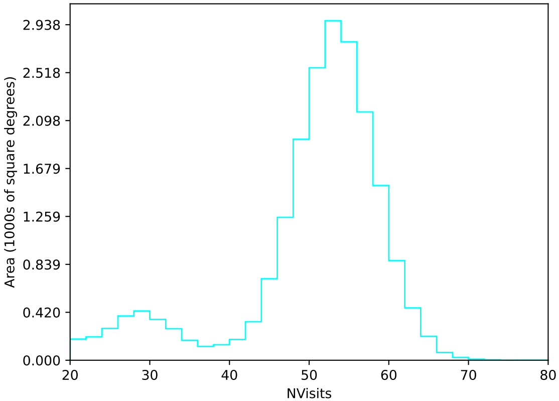
too_elab_heavy_r32_d3_griz_v3.4_10yrs All sky u band: NVisits
