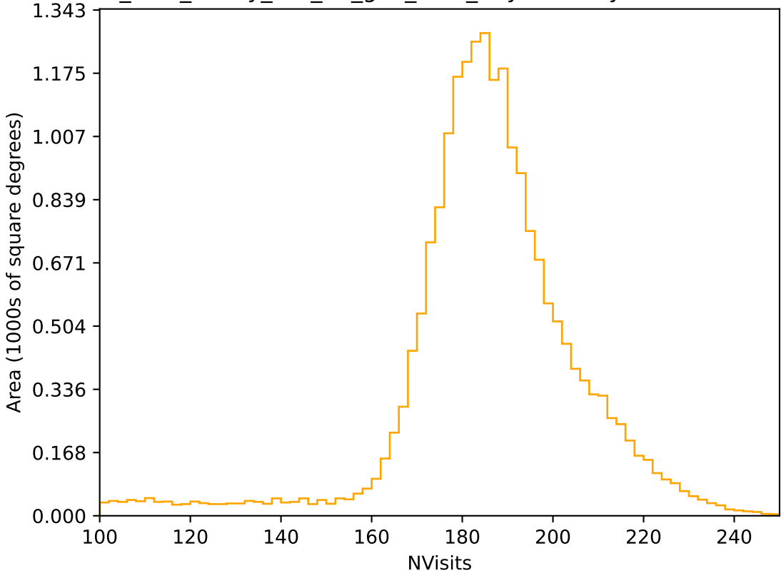
too_elab_heavy_r32_d3_griz_v3.4_10yrs All sky r band: NVisits
