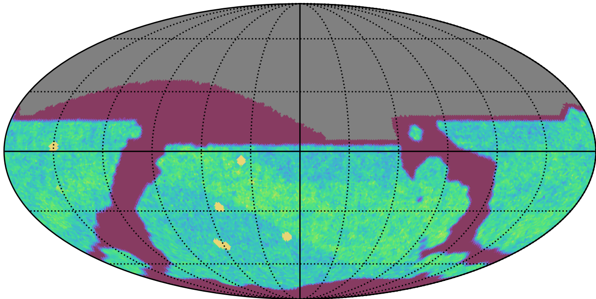
too_elab_heavy_r32_d3_griz_v3.4_10yrs All sky i band: NVisits
