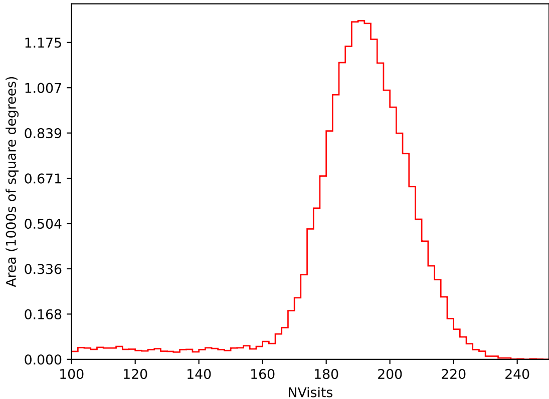
too_elab_heavy_r32_d3_griz_v3.4_10yrs All sky i band: NVisits
