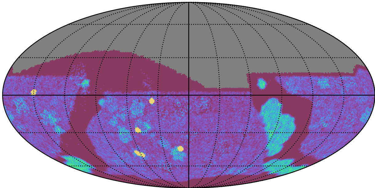
too_elab_heavy_r32_d3_griz_v3.4_10yrs All sky g band: NVisits
