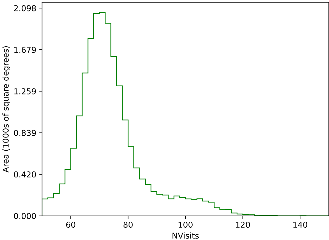
too_elab_heavy_r32_d3_griz_v3.4_10yrs All sky g band: NVisits
