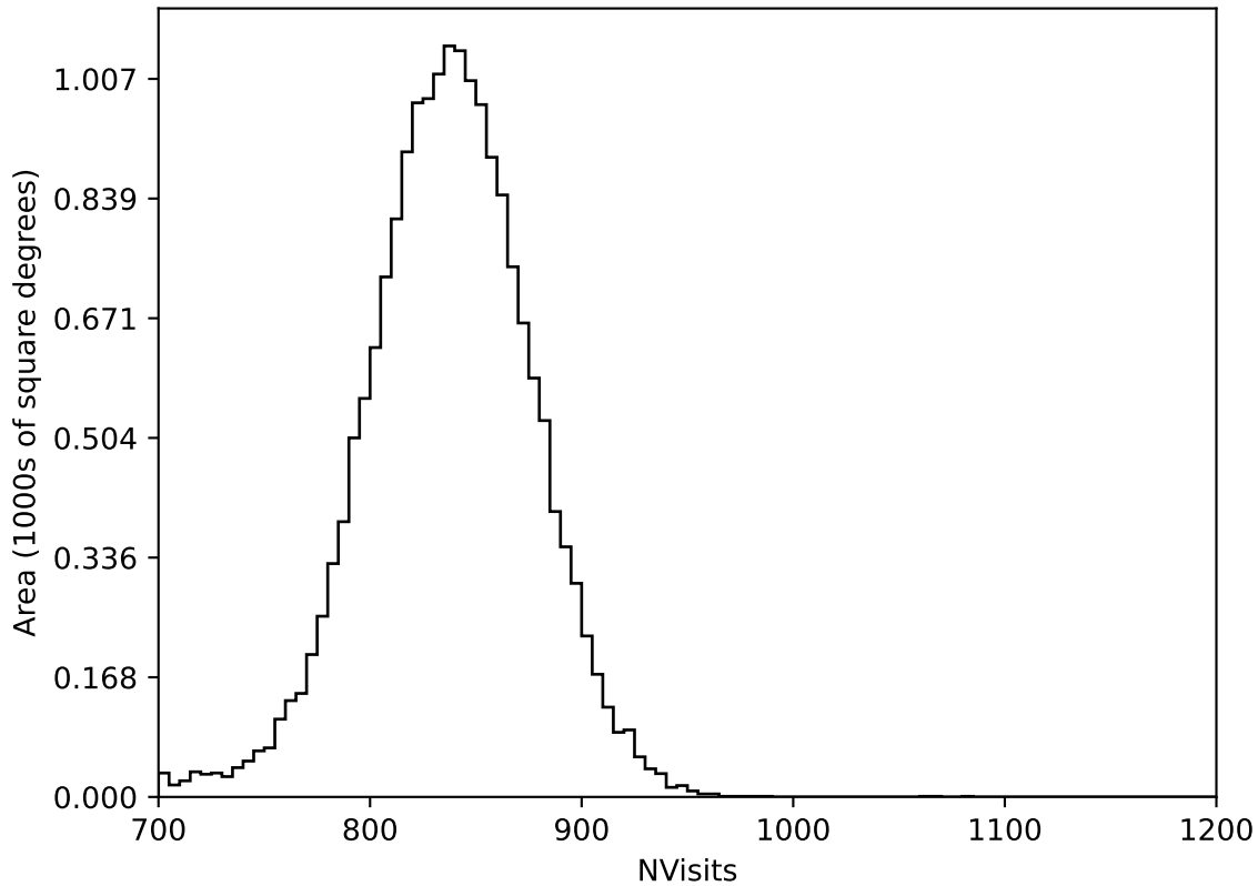
too_elab_heavy_r32_d3_griz_v3.4_10yrs All sky all bands: NVisits
