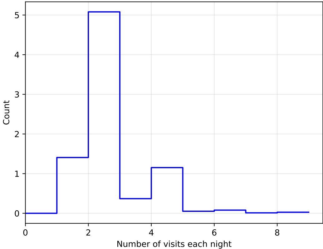
too_elab_heavy_r32_d3_griz_v3.4_10yrs WFD: NVisitsPerNight 1e6
