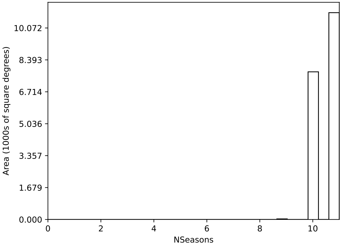
too_elab_heavy_r32_d3_griz_v3.4_10yrs WFD all bands: NSeasons
