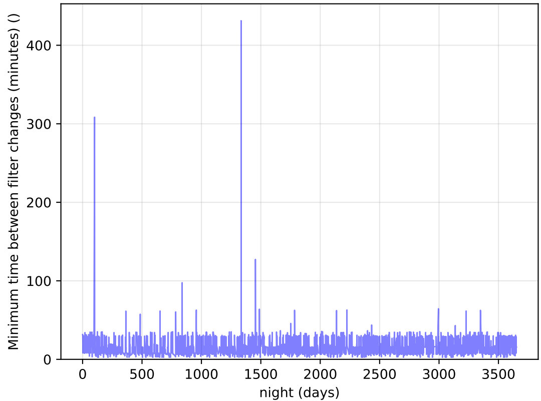
too_elab_heavy_r32_d3_griz_v3.4_10yrs Per Night: Minimum time between filter changes (minutes)
