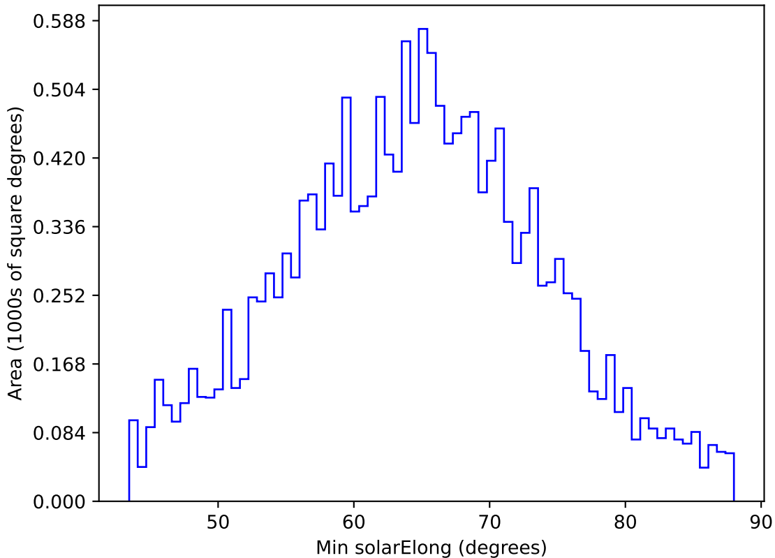
too_elab_heavy_r32_d3_griz_v3.4_10yrs WFD y band: Min solarElong
