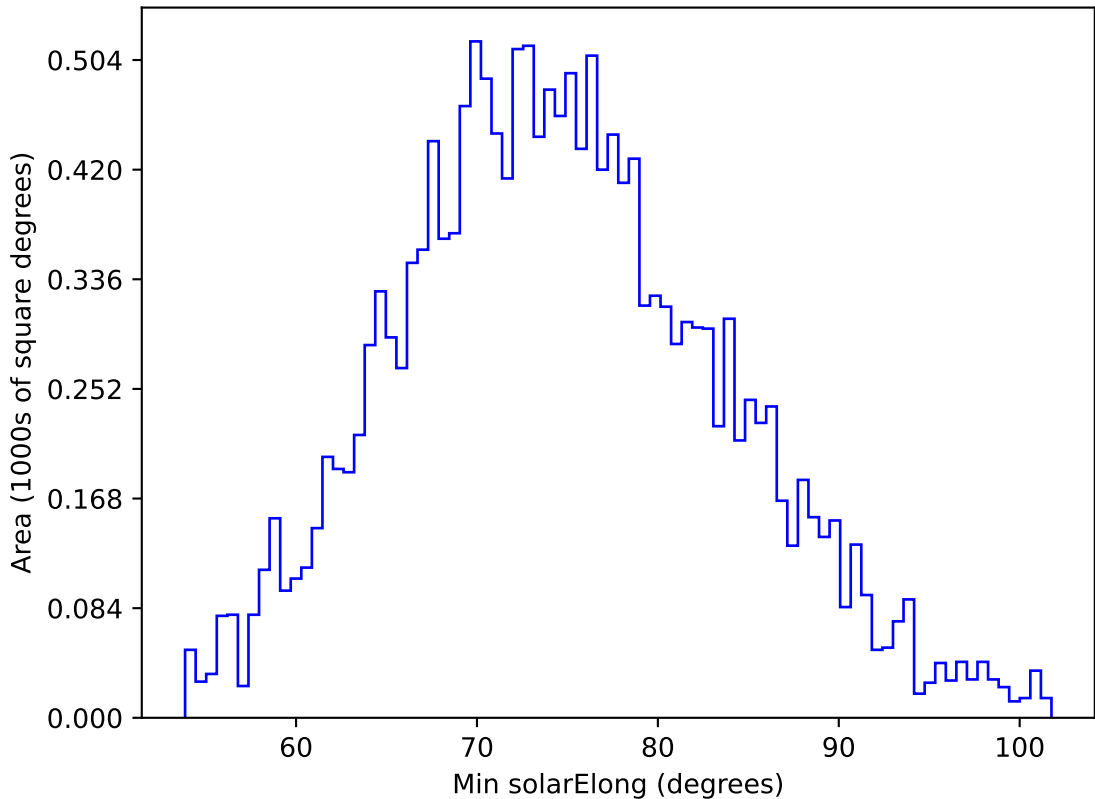
too_elab_heavy_r32_d3_griz_v3.4_10yrs WFD g band: Min solarElong
