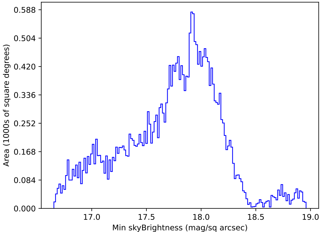
too_elab_heavy_r32_d3_griz_v3.4_10yrs Yr 1 all bands: Min skyBrightness
