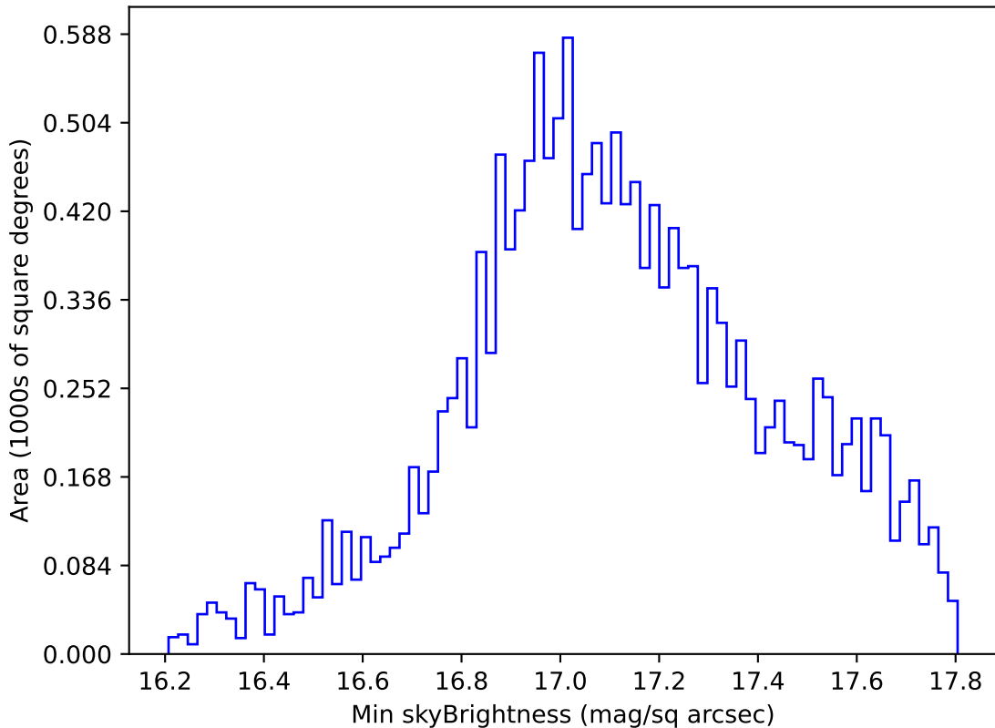
too_elab_heavy_r32_d3_griz_v3.4_10yrs WFD y band: Min skyBrightness
