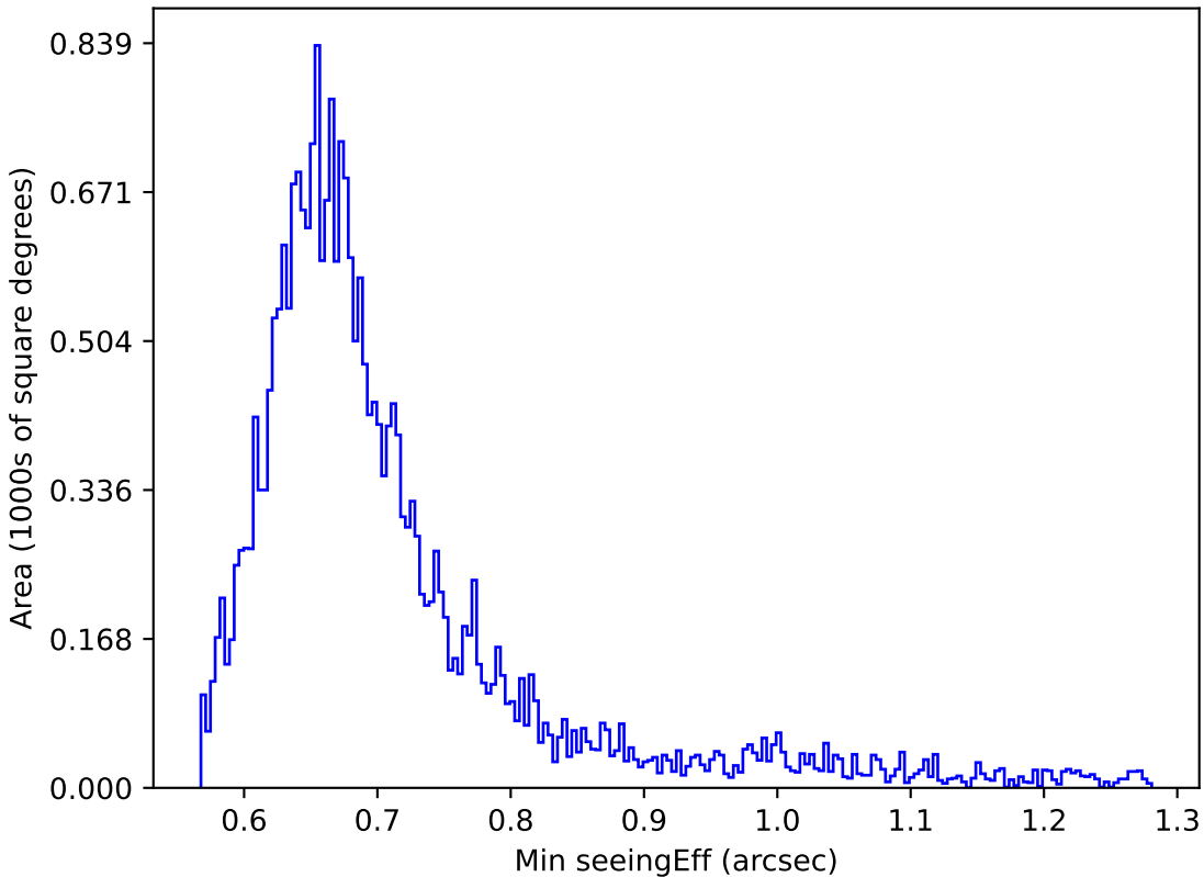
too_elab_heavy_r32_d3_griz_v3.4_10yrs Yr 1 i band: Min seeingEff
