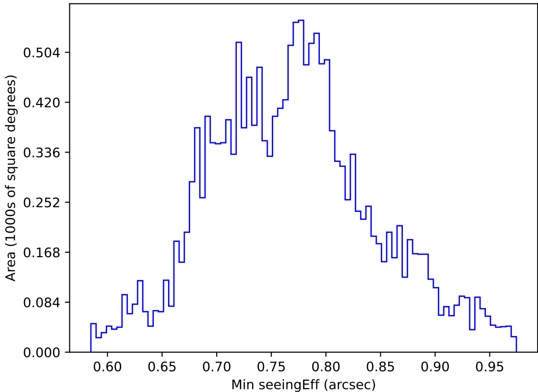
too_elab_heavy_r32_d3_griz_v3.4_10yrs WFD u band: Min seeingEff
