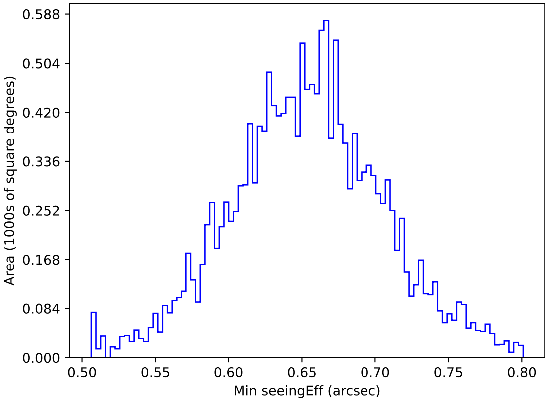
too_elab_heavy_r32_d3_griz_v3.4_10yrs WFD g band: Min seeingEff
