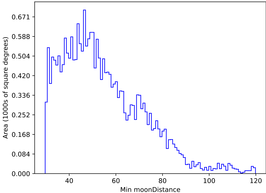
too_elab_heavy_r32_d3_griz_v3.4_10yrs All sky u band: Min moonDistance
