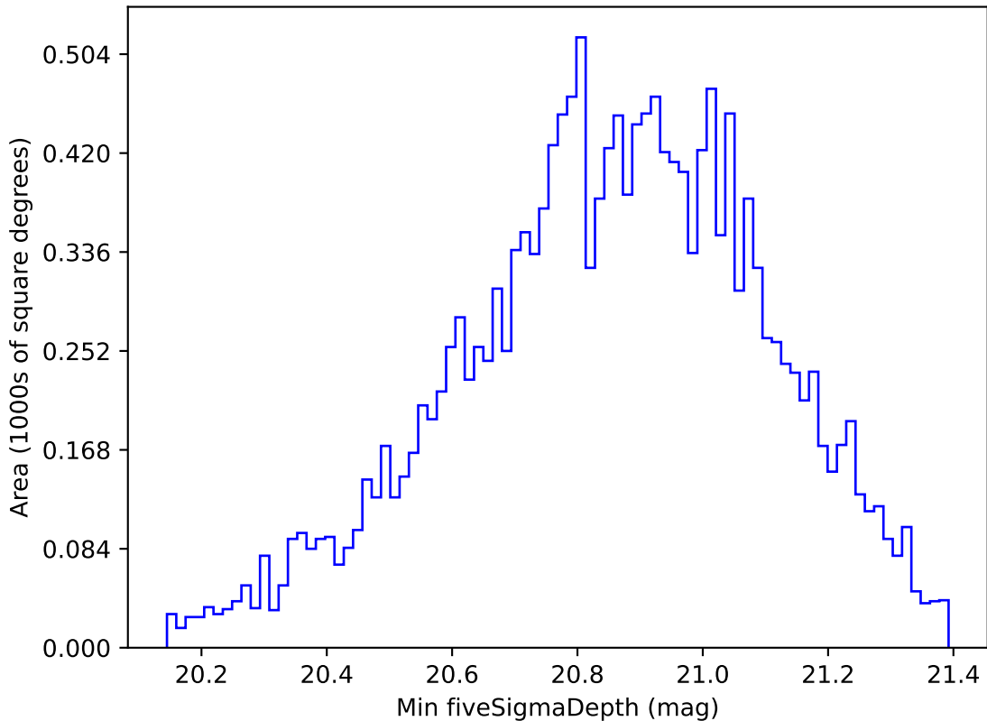
too_elab_heavy_r32_d3_griz_v3.4_10yrs WFD y band: Min fiveSigmaDepth
