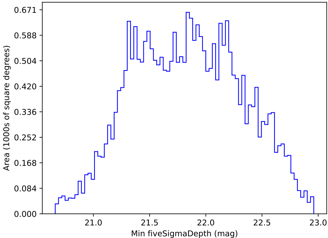
too_elab_heavy_r32_d3_griz_v3.4_10yrs All sky i band: Min fiveSigmaDepth
