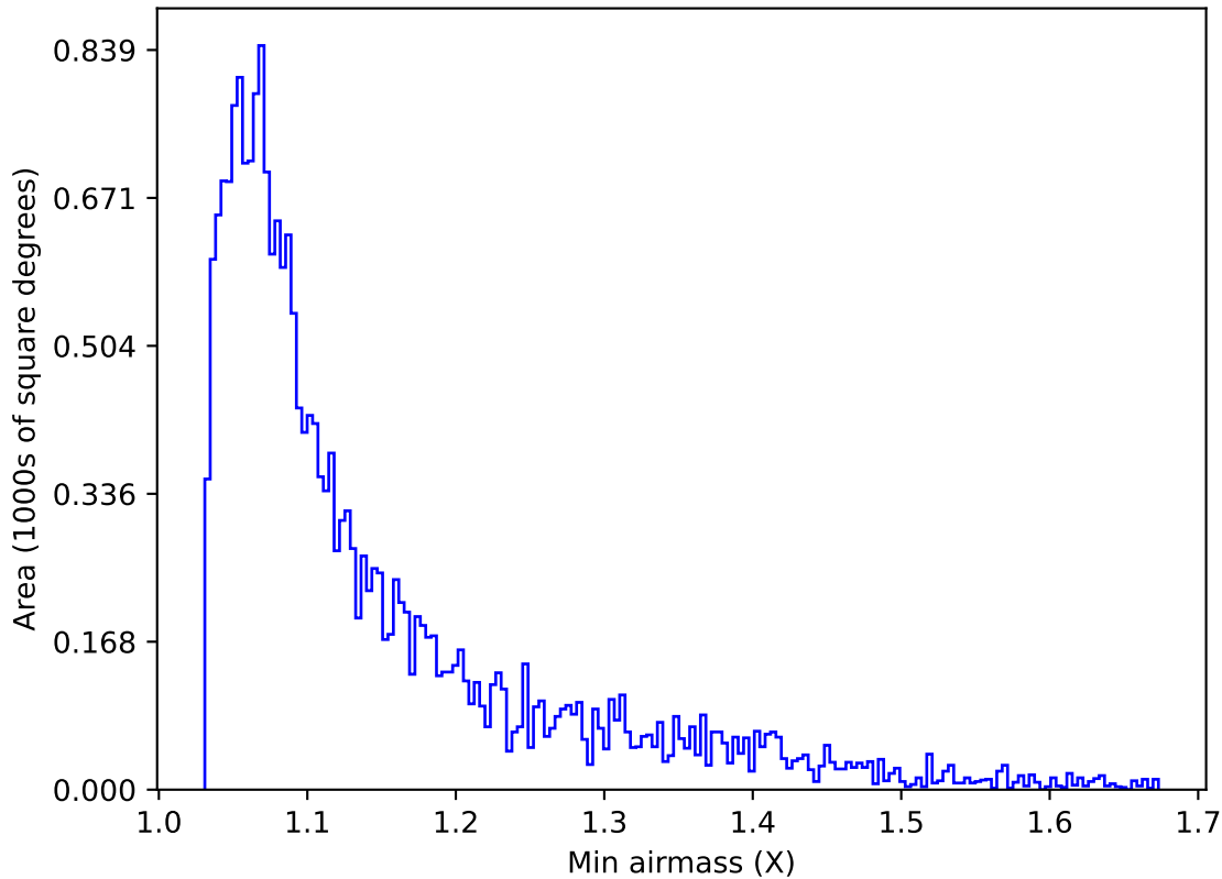
too_elab_heavy_r32_d3_griz_v3.4_10yrs Yr 1 u band: Min airmass
