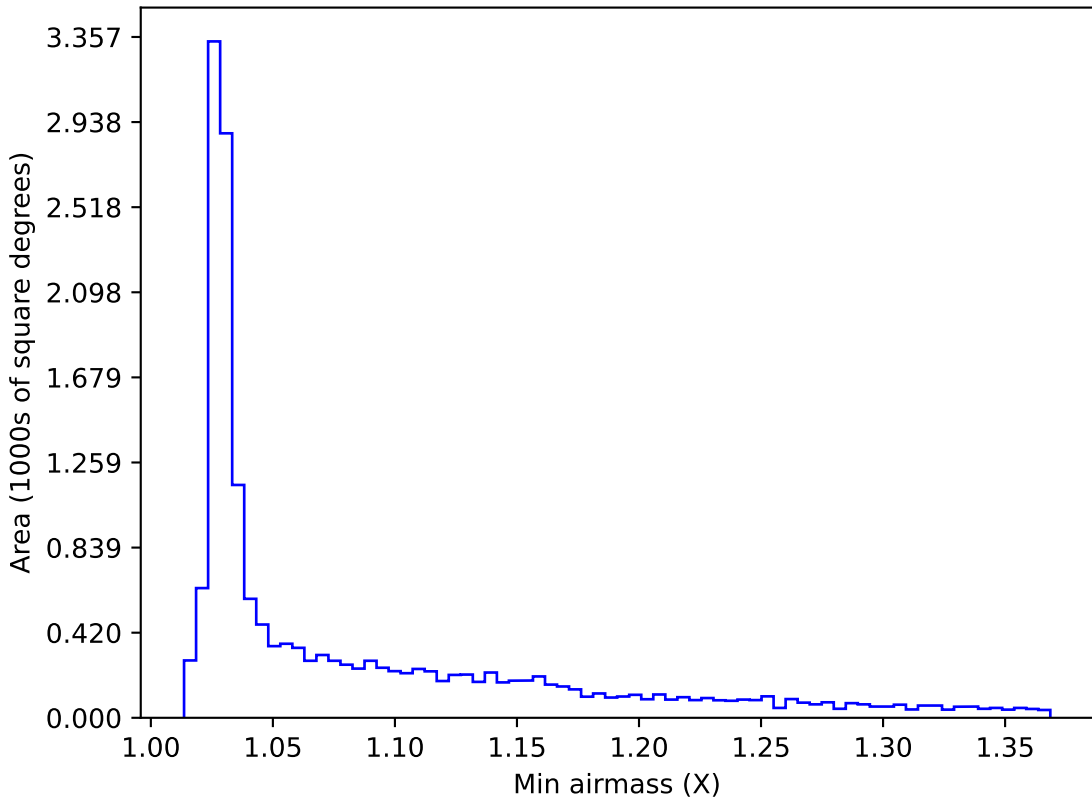
too_elab_heavy_r32_d3_griz_v3.4_10yrs WFD z band: Min airmass
