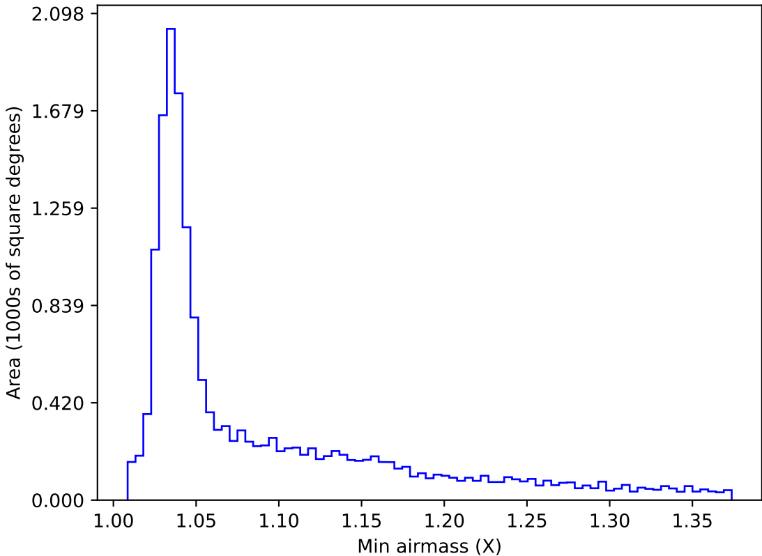
too_elab_heavy_r32_d3_griz_v3.4_10yrs WFD g band: Min airmass
