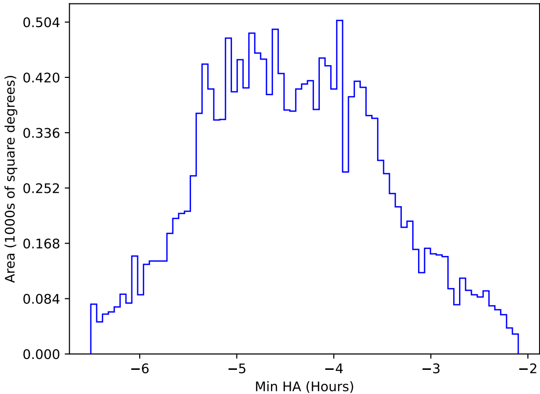
too_elab_heavy_r32_d3_griz_v3.4_10yrs WFD z band: Min HA
