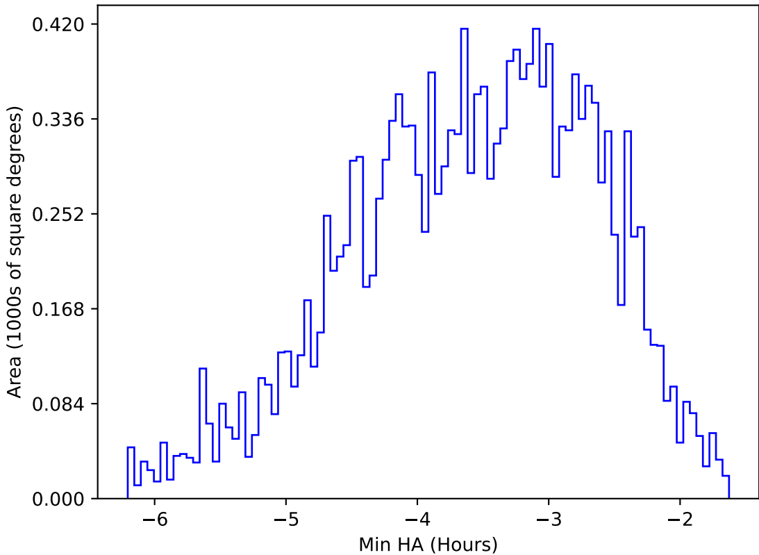
too_elab_heavy_r32_d3_griz_v3.4_10yrs WFD y band: Min HA
