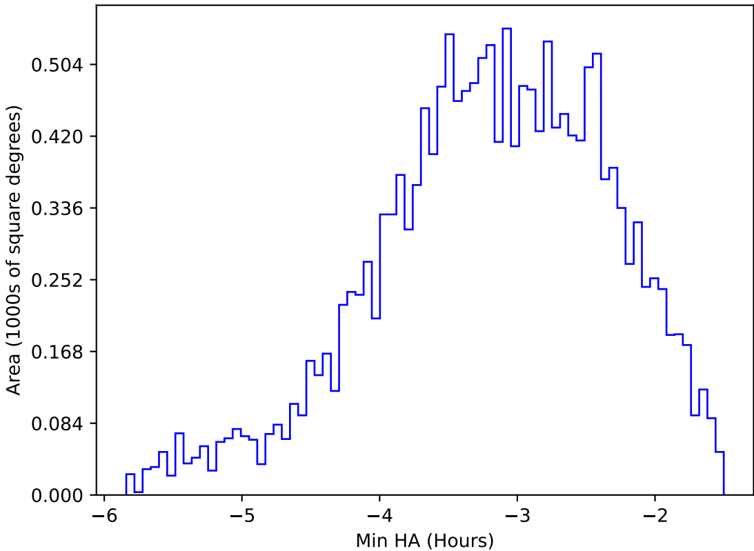
too_elab_heavy_r32_d3_griz_v3.4_10yrs WFD u band: Min HA
