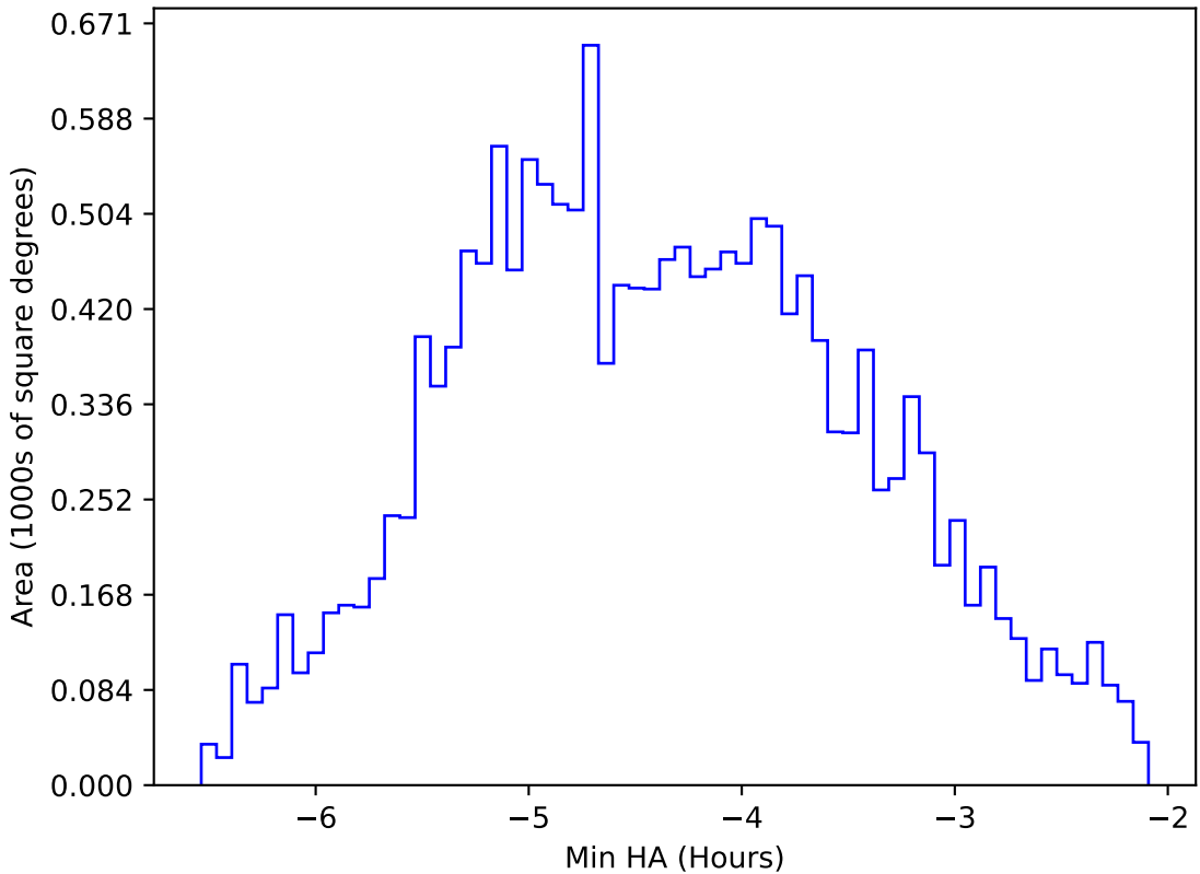
too_elab_heavy_r32_d3_griz_v3.4_10yrs WFD i band: Min HA
