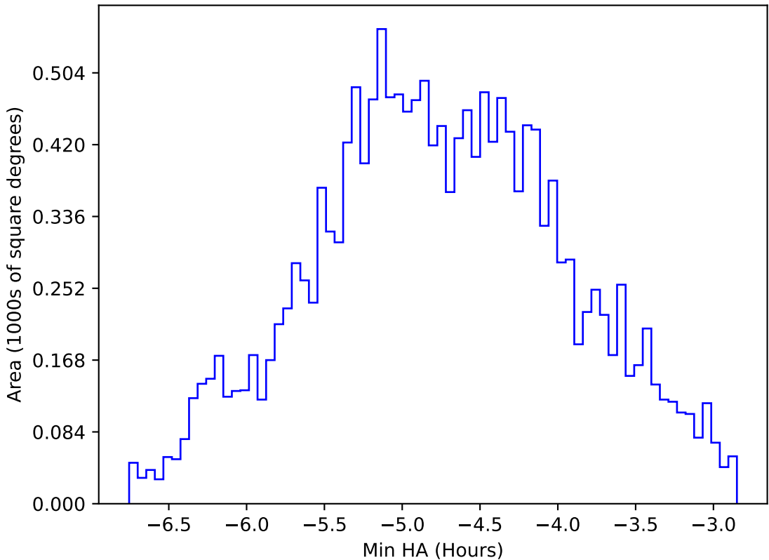
too_elab_heavy_r32_d3_griz_v3.4_10yrs WFD all bands: Min HA
