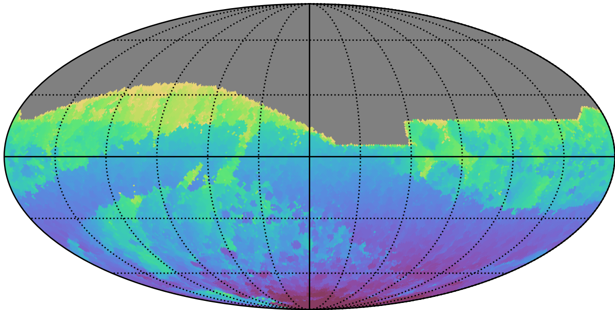
too_elab_heavy_r32_d3_griz_v3.4_10yrs All sky r band: Min HA
